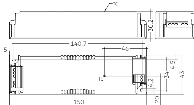
Without strain-relief
